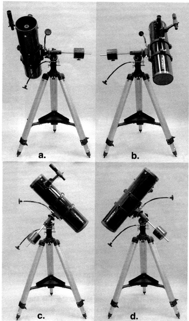
Figure 7. This illustration shows the telescope pointed in the four cardinal directions: (a) north, (b) south, (c) east, (d) west. Note that the tripod and mount have not been moved; only the telescope tube has been moved on the R.A. and Dec. axes.
