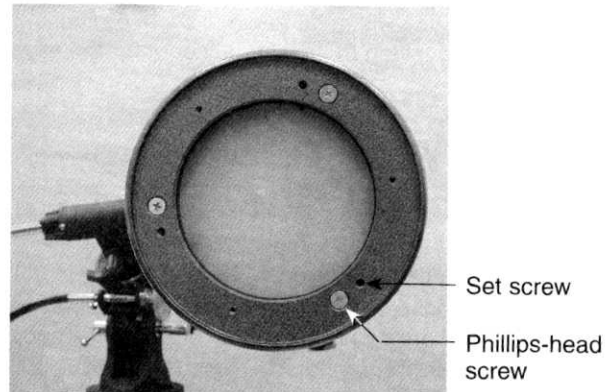
Figure 11. The back end of the optical tube (bottom of the primary mirror cell). The three pairs of set screws and Phillips-head screws adjust the tilt of the primary mirror.
